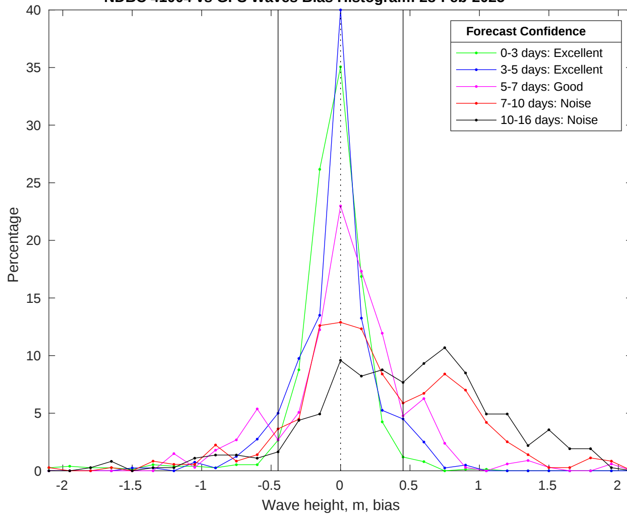
NDBC 41004 vs GFS Waves Bias Histogram: 28-Feb-2025
