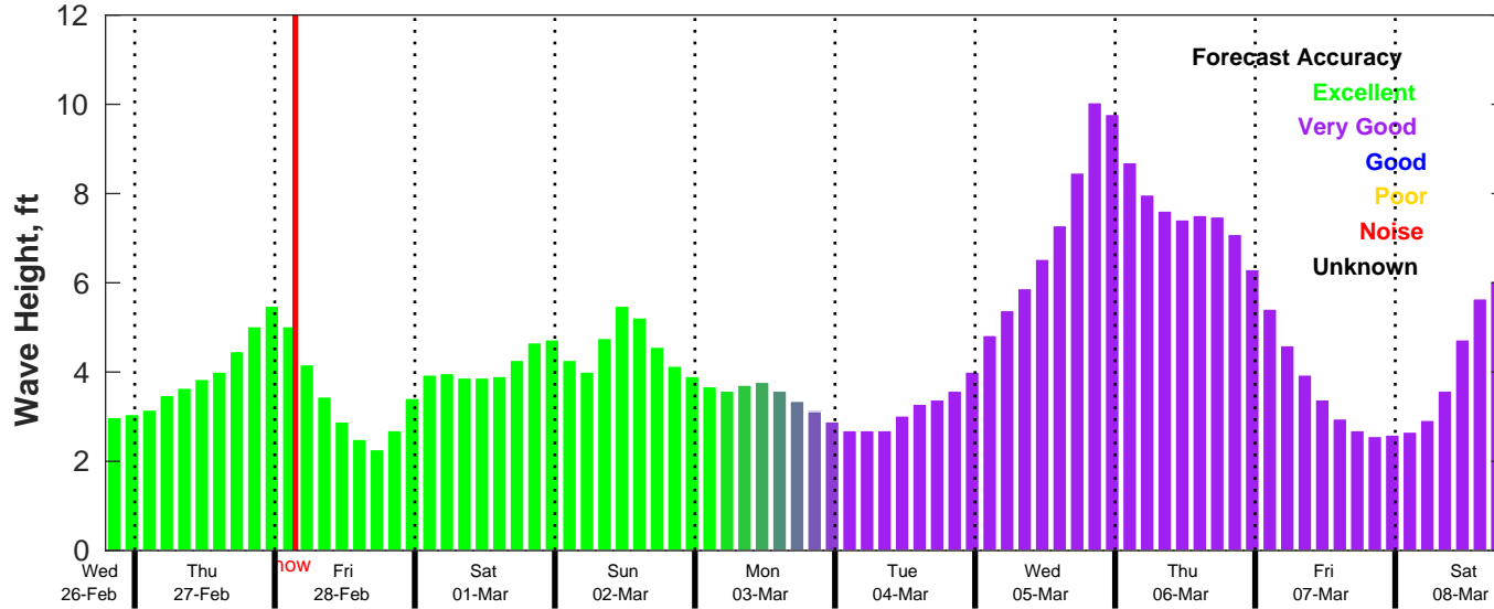
CMEMS Wave Forecast for NDBC 41004 from 26-Feb-2025 19:00:00 to 08-Mar-2025 19:00:00
