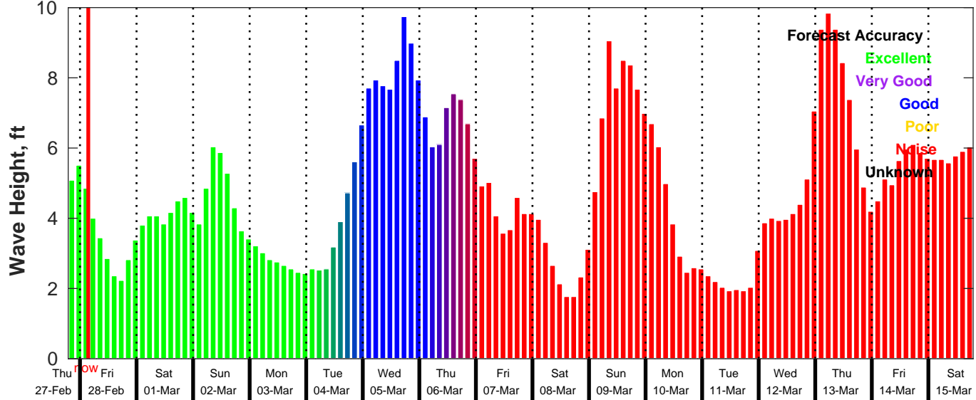
GFS Wave Forecast for NDBC 41004 from 27-Feb-2025 19:00:00 to 15-Mar-2025 19:00:00
