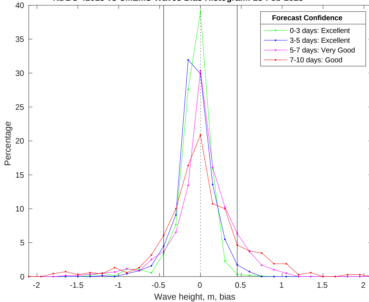
NDBC 41013 vs CMEMS Waves Bias Histogram: 28-Feb-2025
