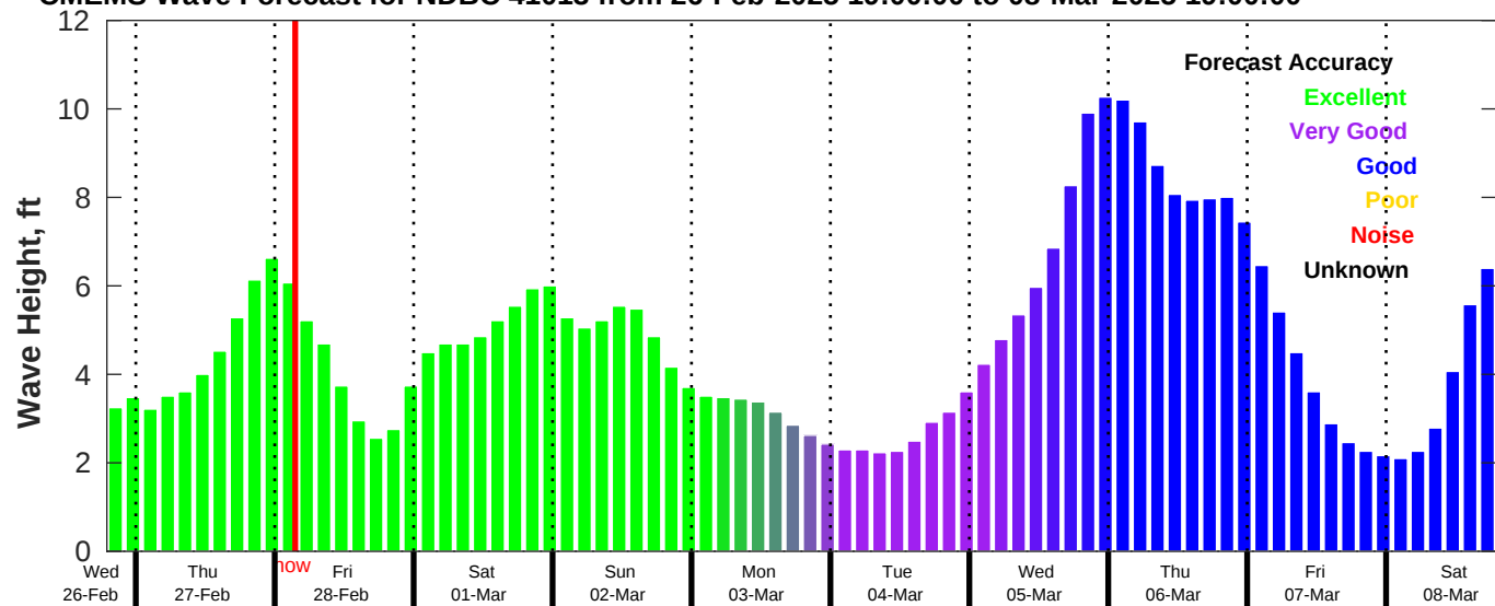
CMEMS Wave Forecast for NDBC 41013 from 26-Feb-2025 19:00:00 to 08-Mar-2025 19:00:00
