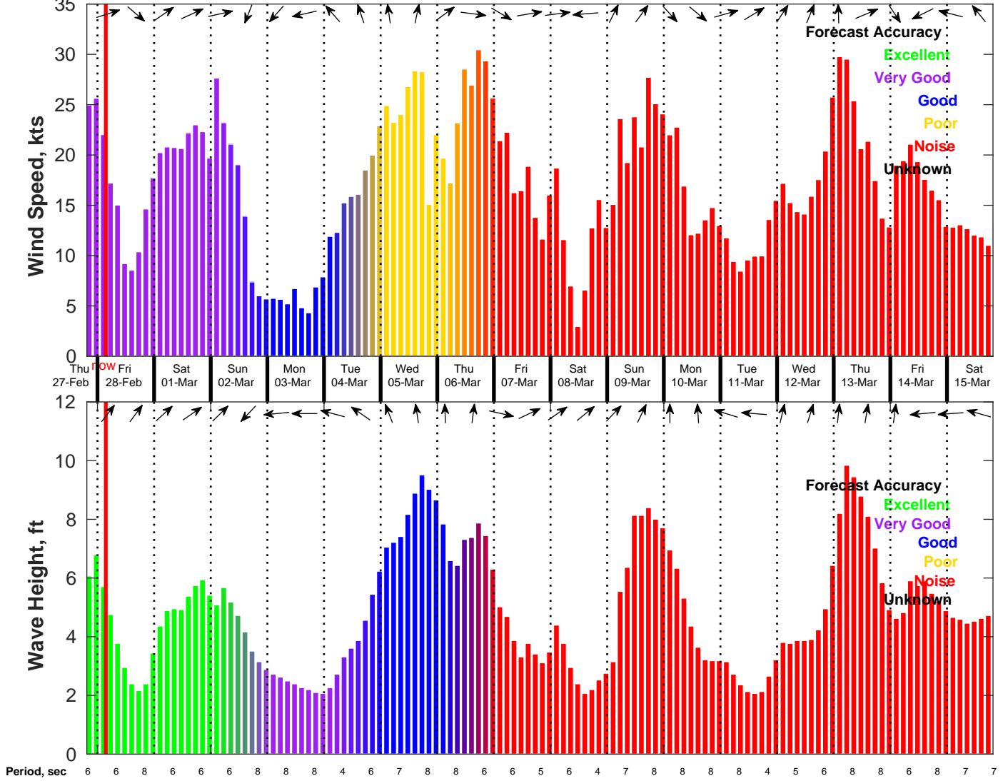
Wind & Wave Forecast for NDBC 41013 from 27-Feb-2025 19:00:00 to 15-Mar-2025 19:00:00
