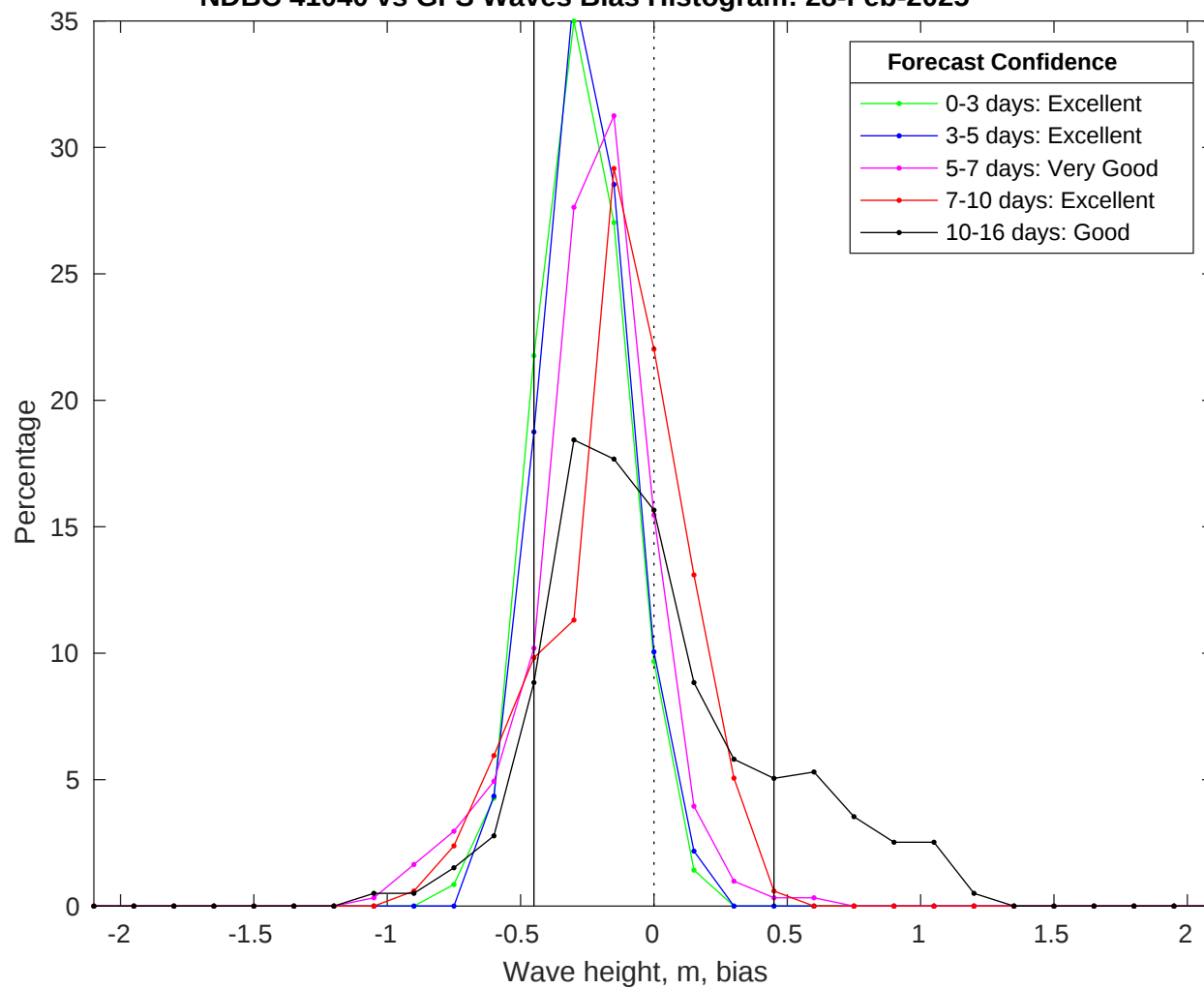
NDBC 41040 vs GFS Waves Bias Histogram: 28-Feb-2025
