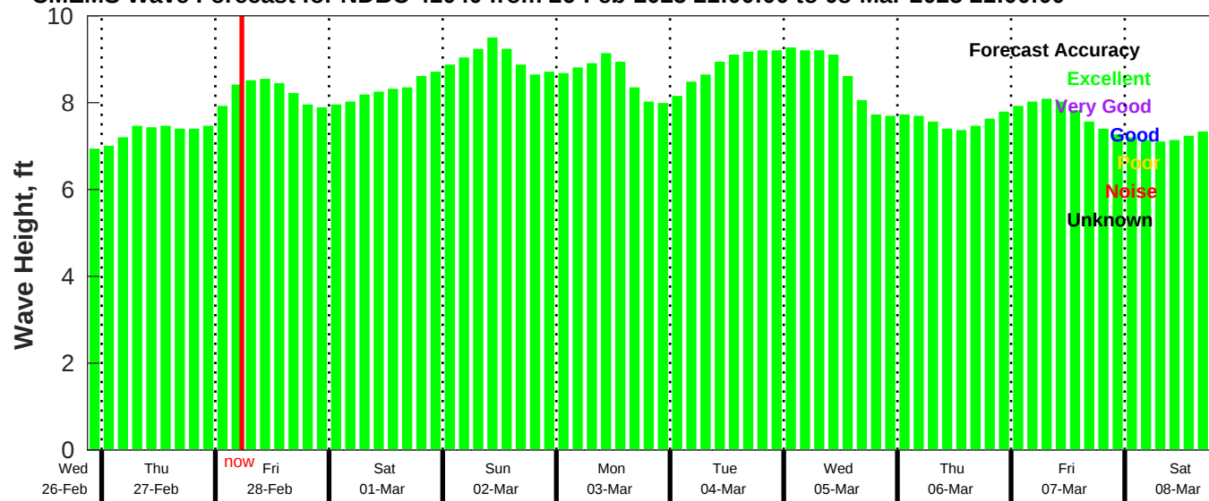
CMEMS Wave Forecast for NDBC 41040 from 26-Feb-2025 21:00:00 to 08-Mar-2025 21:00:00
