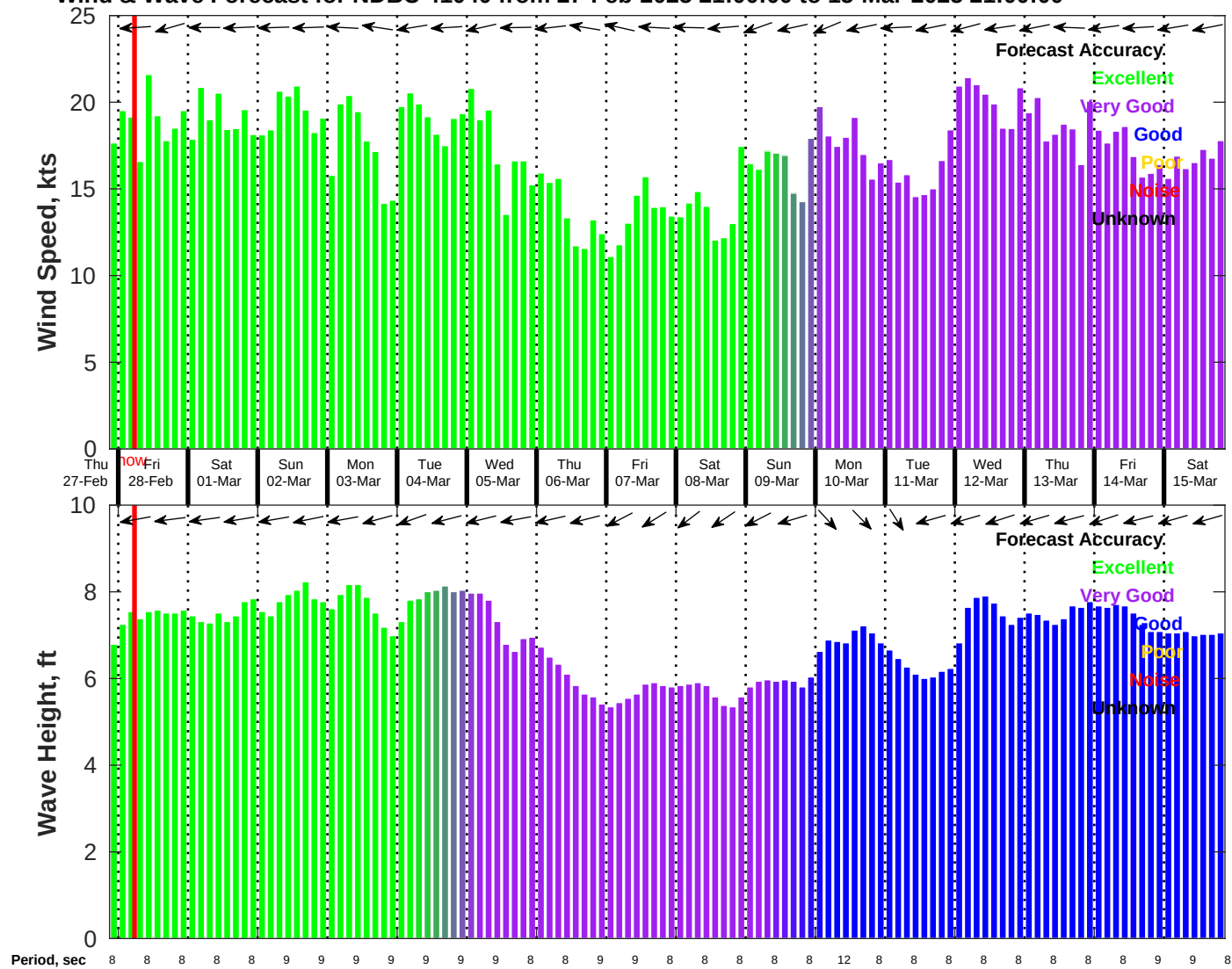
Wind & Wave Forecast for NDBC 41040 from 27-Feb-2025 21:00:00 to 15-Mar-2025 21:00:00
