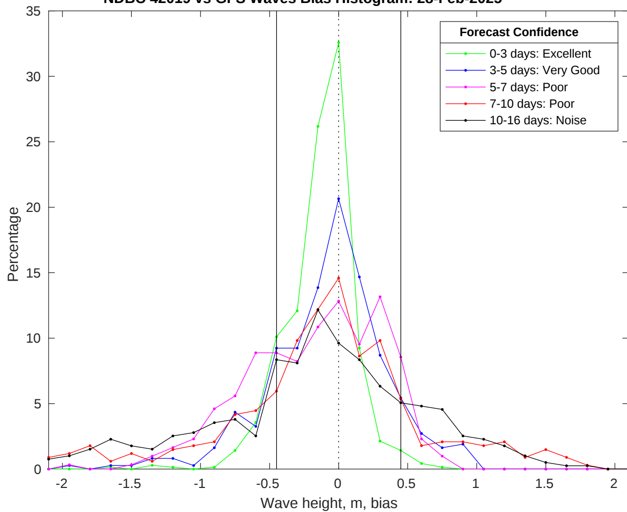
NDBC 42019 vs GFS Waves Bias Histogram: 28-Feb-2025
