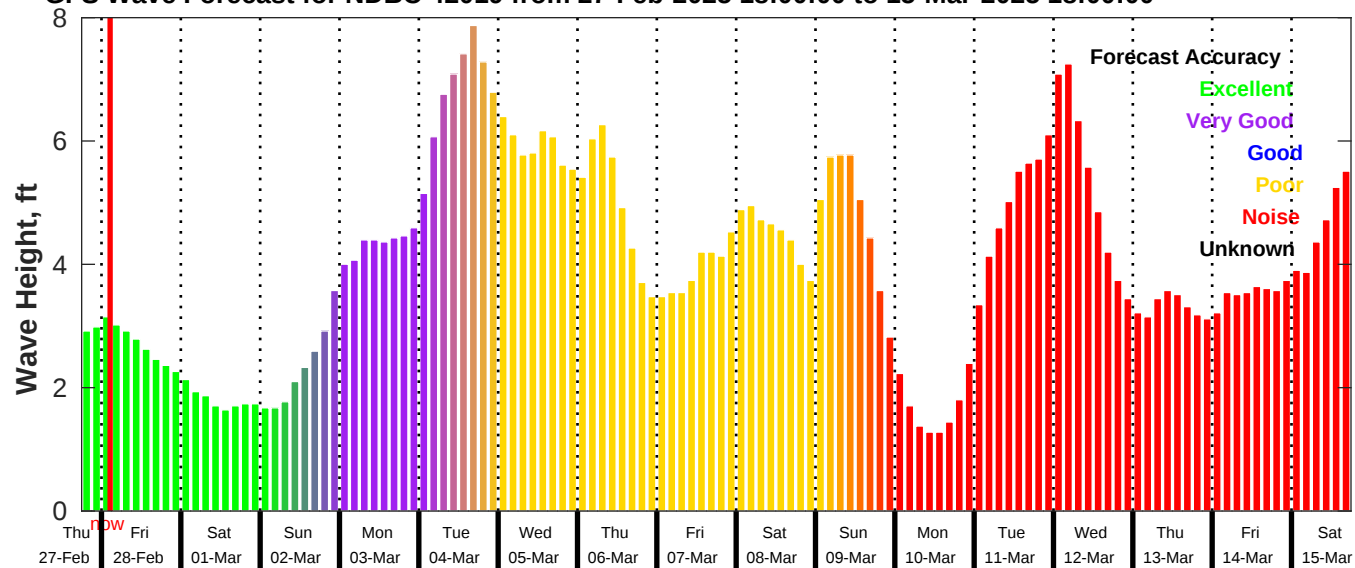
GFS Wave Forecast for NDBC 42019 from 27-Feb-2025 18:00:00 to 15-Mar-2025 18:00:00
