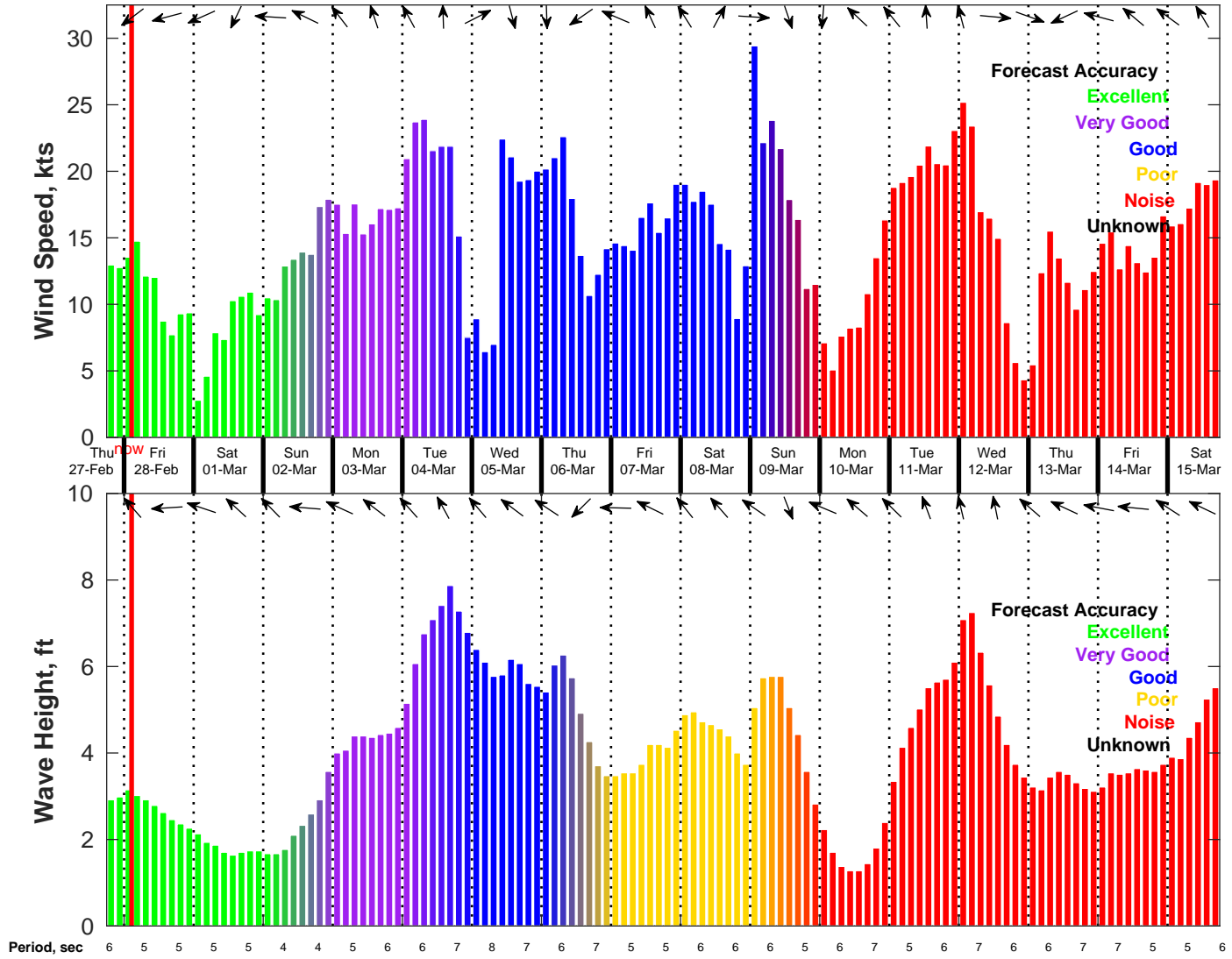
Wind & Wave Forecast for NDBC 42019 from 27-Feb-2025 18:00:00 to 15-Mar-2025 18:00:00
