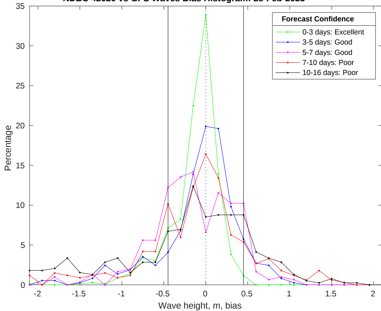
NDBC 42020 vs GFS Waves Bias Histogram: 28-Feb-2025
