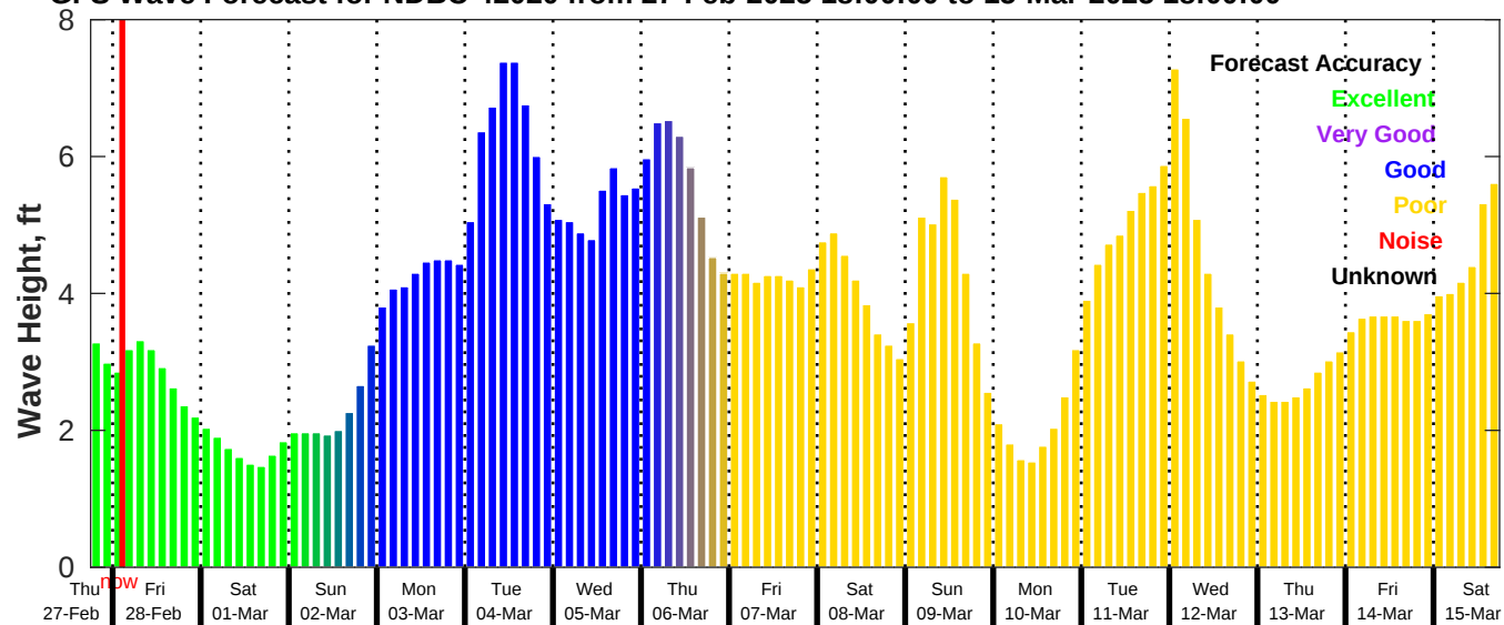
GFS Wave Forecast for NDBC 42020 from 27-Feb-2025 18:00:00 to 15-Mar-2025 18:00:00
