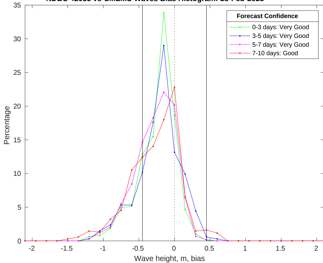
NDBC 42035 vs CMEMS Waves Bias Histogram: 28-Feb-2025
