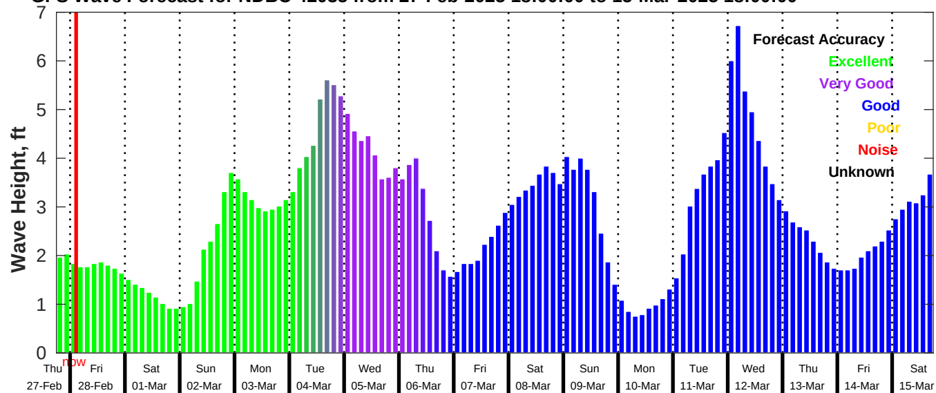
GFS Wave Forecast for NDBC 42035 from 27-Feb-2025 18:00:00 to 15-Mar-2025 18:00:00
