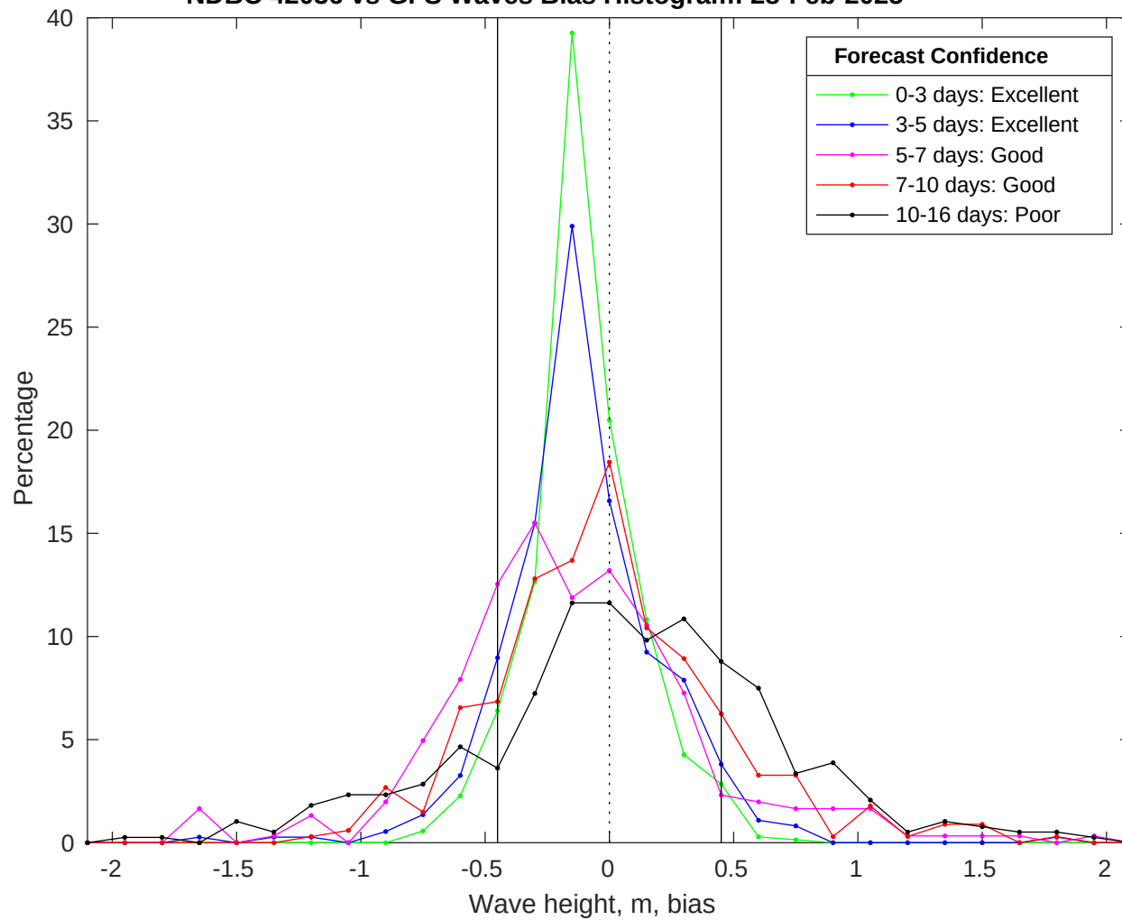
NDBC 42036 vs GFS Waves Bias Histogram: 28-Feb-2025
