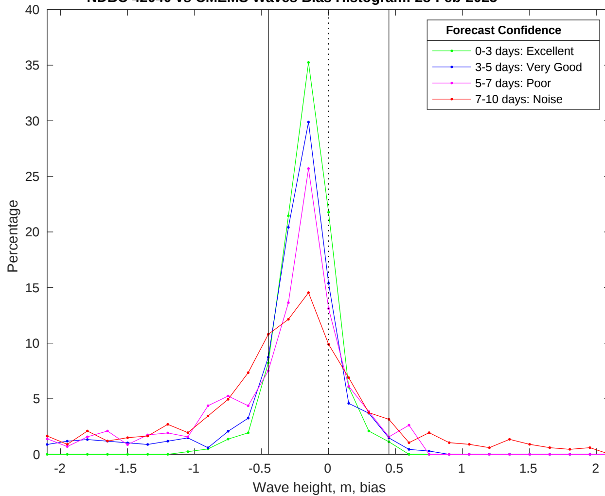
NDBC 42040 vs CMEMS Waves Bias Histogram: 28-Feb-2025
