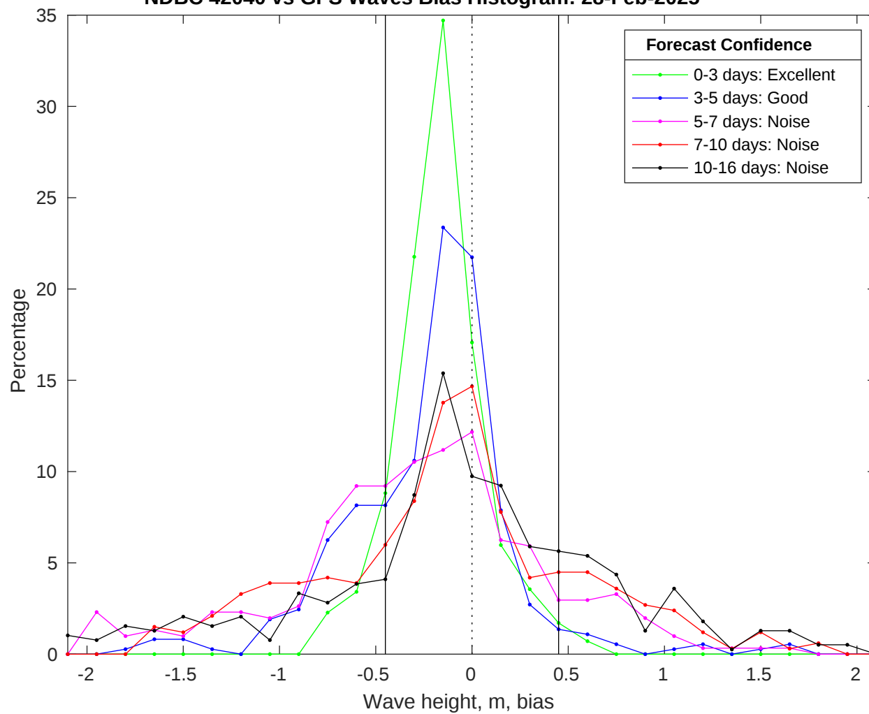
NDBC 42040 vs GFS Waves Bias Histogram: 28-Feb-2025
