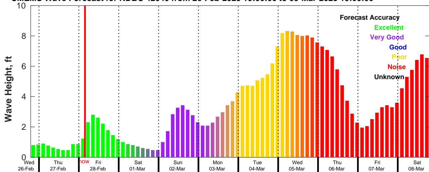
CMEMS Wave Forecast for NDBC 42040 from 26-Feb-2025 19:00:00 to 08-Mar-2025 19:00:00
