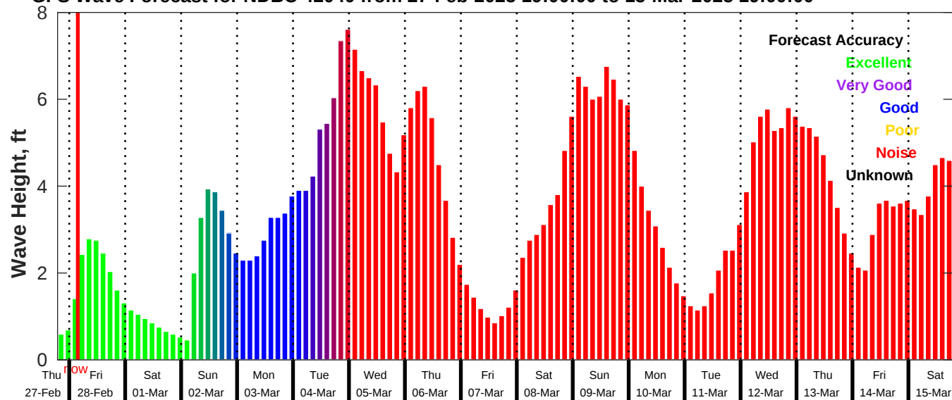
GFS Wave Forecast for NDBC 42040 from 27-Feb-2025 19:00:00 to 15-Mar-2025 19:00:00
