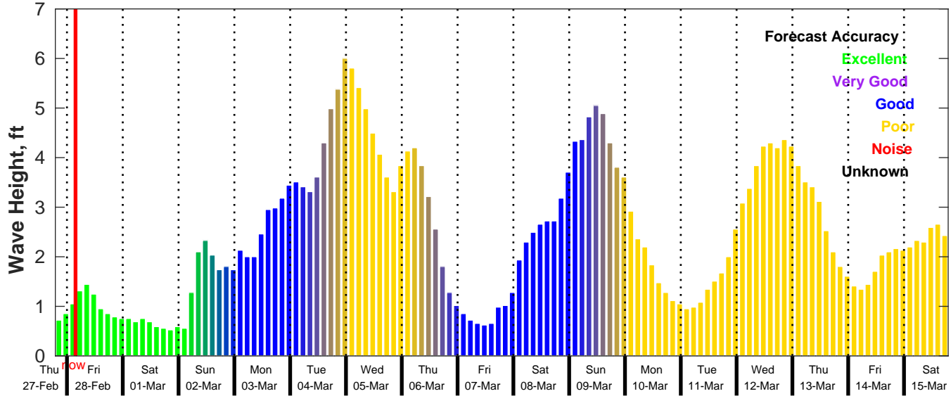
GFS Wave Forecast for NDBC 42084 from 27-Feb-2025 19:00:00 to 15-Mar-2025 19:00:00
