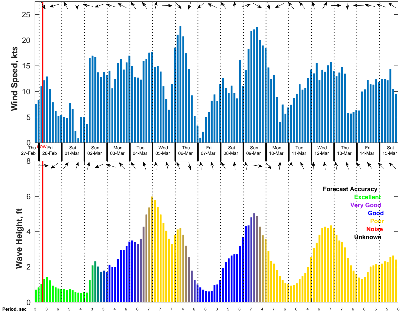
Wind & Wave Forecast for NDBC 42084 from 27-Feb-2025 19:00:00 to 15-Mar-2025 19:00:00
