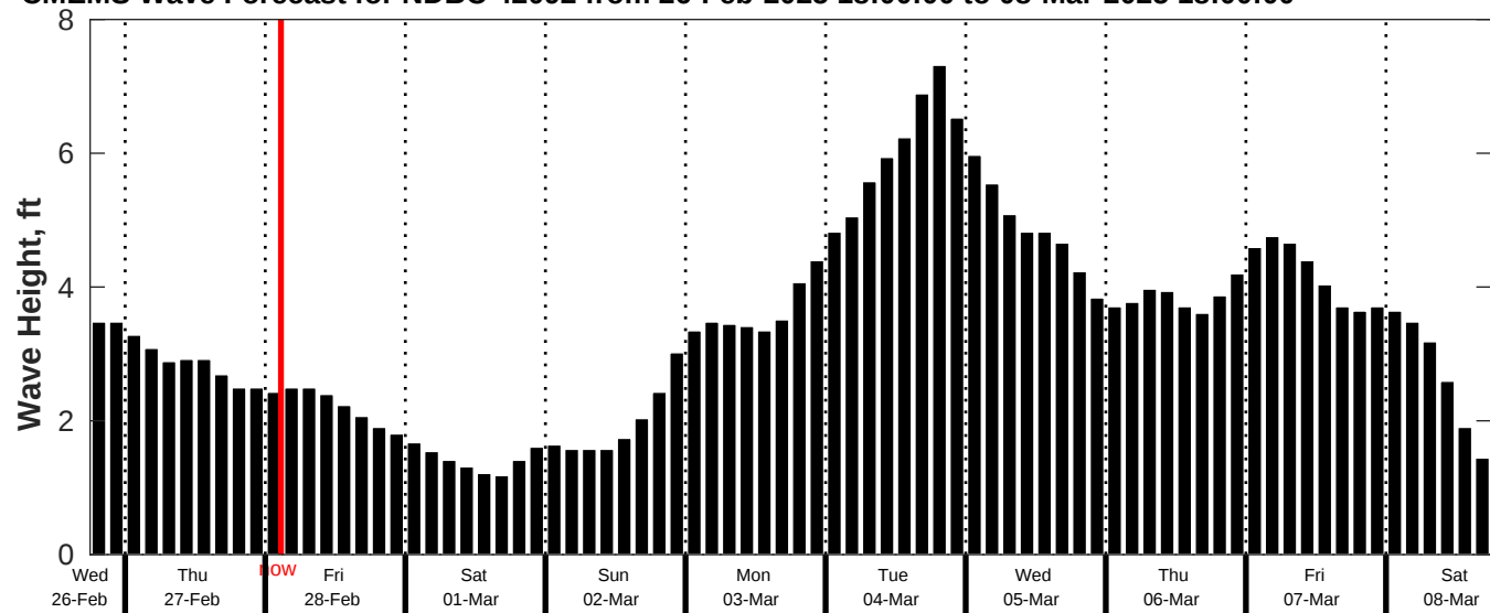
CMEMS Wave Forecast for NDBC 42092 from 26-Feb-2025 18:00:00 to 08-Mar-2025 18:00:00
