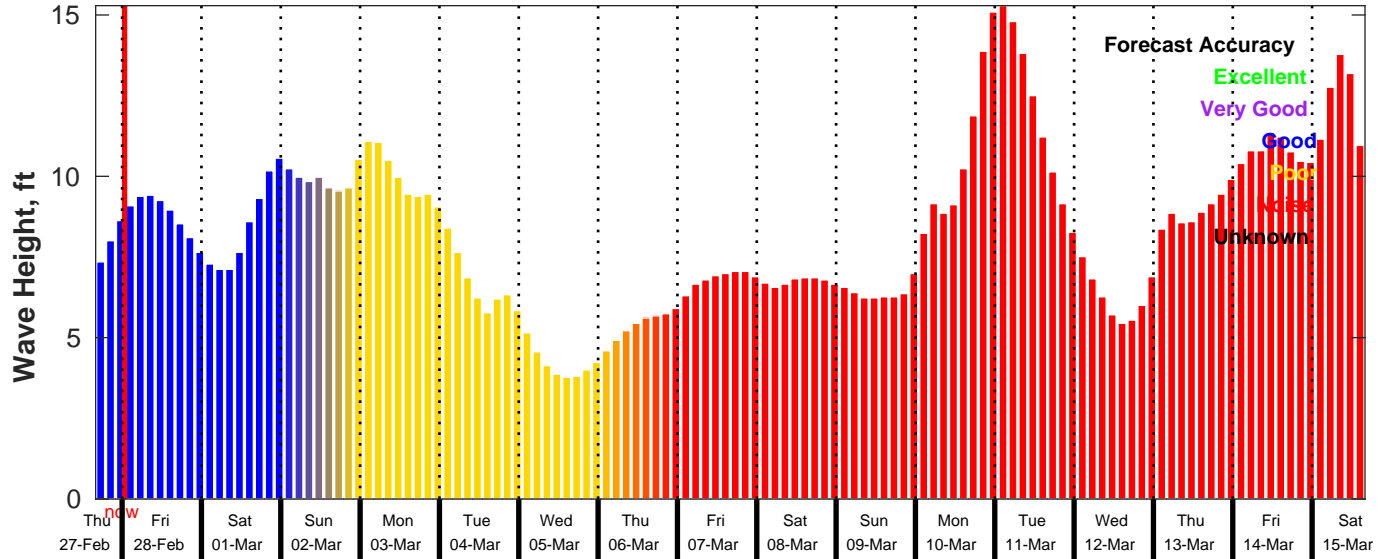
GFS Wave Forecast for NDBC 46011 from 27-Feb-2025 16:00:00 to 15-Mar-2025 16:00:00
