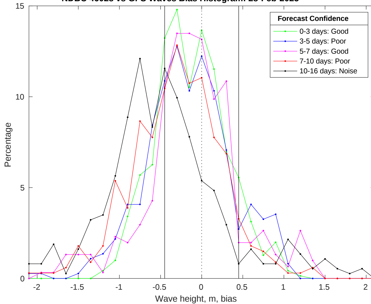
NDBC 46028 vs GFS Waves Bias Histogram: 28-Feb-2025
