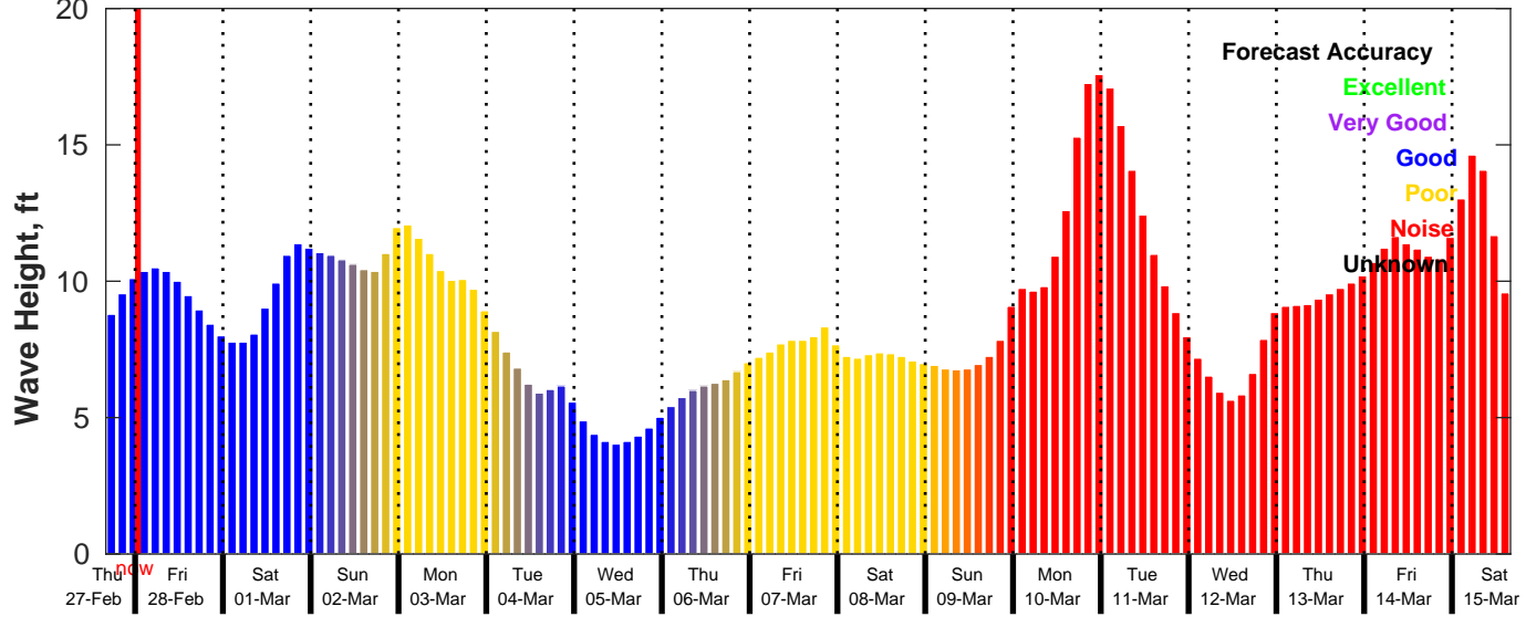
GFS Wave Forecast for NDBC 46028 from 27-Feb-2025 16:00:00 to 15-Mar-2025 16:00:00
