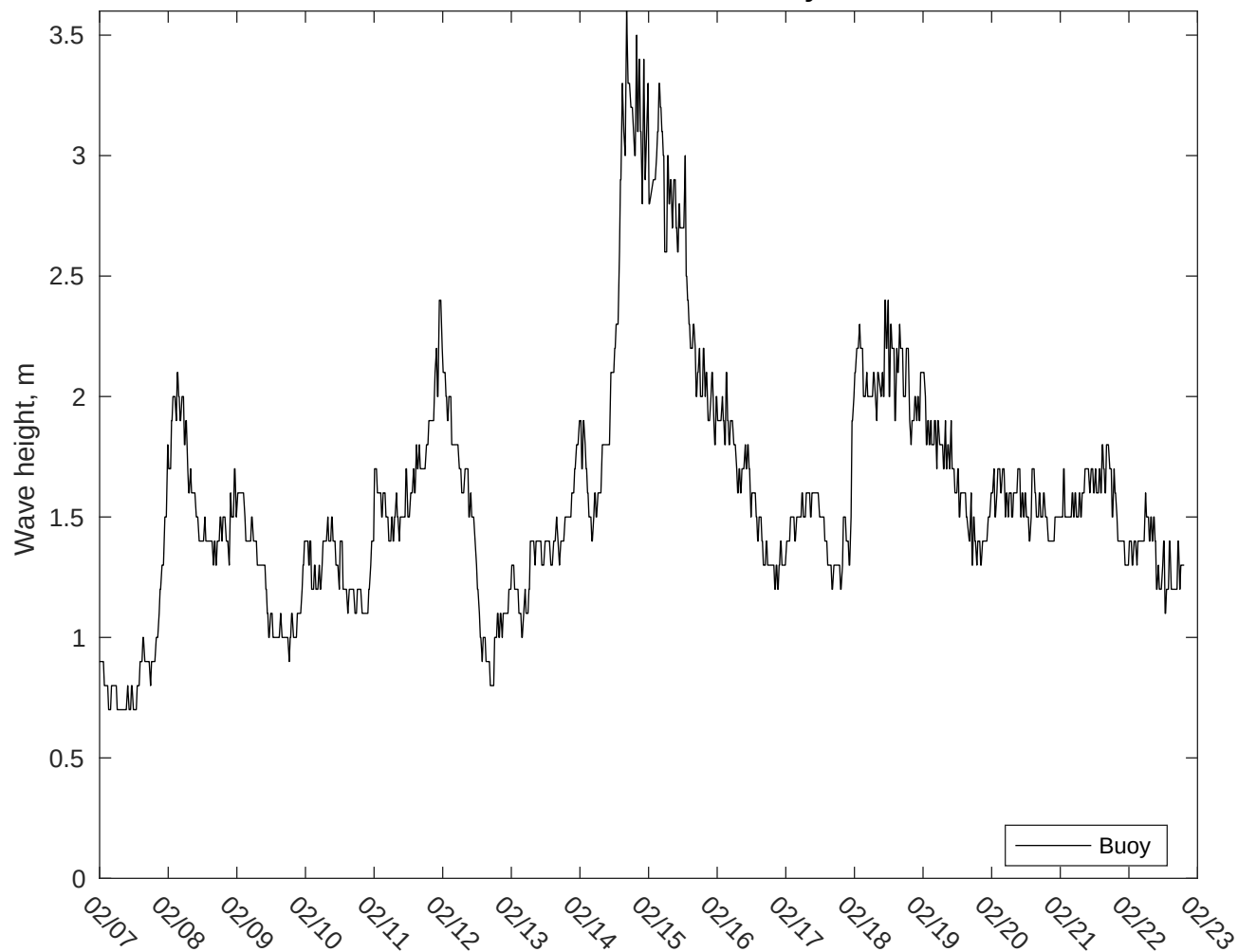
NDBC 46053 vs CMEMS Waves: 10 to 16 day forecast
