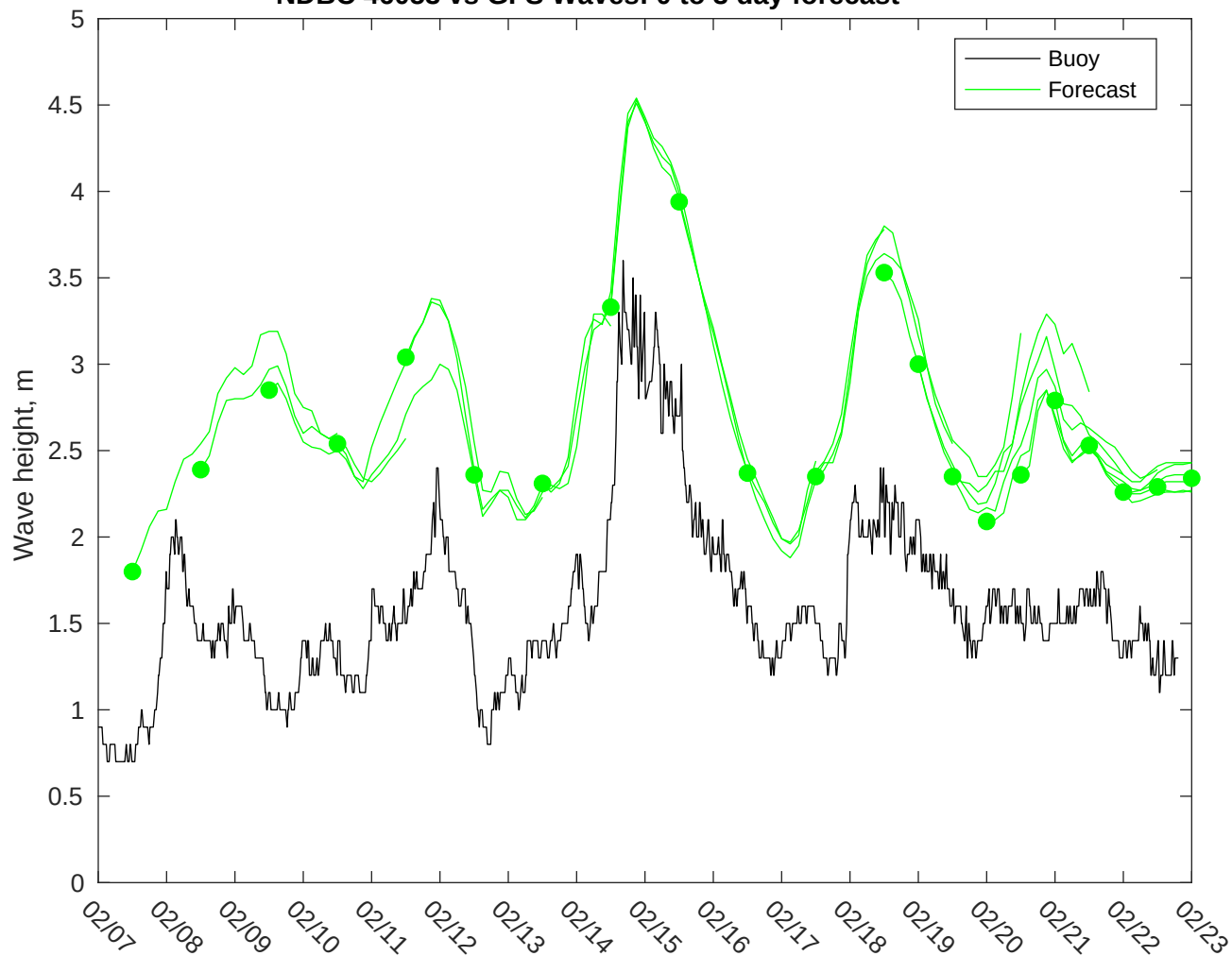
NDBC 46053 vs GFS Waves: 0 to 3 day forecast
