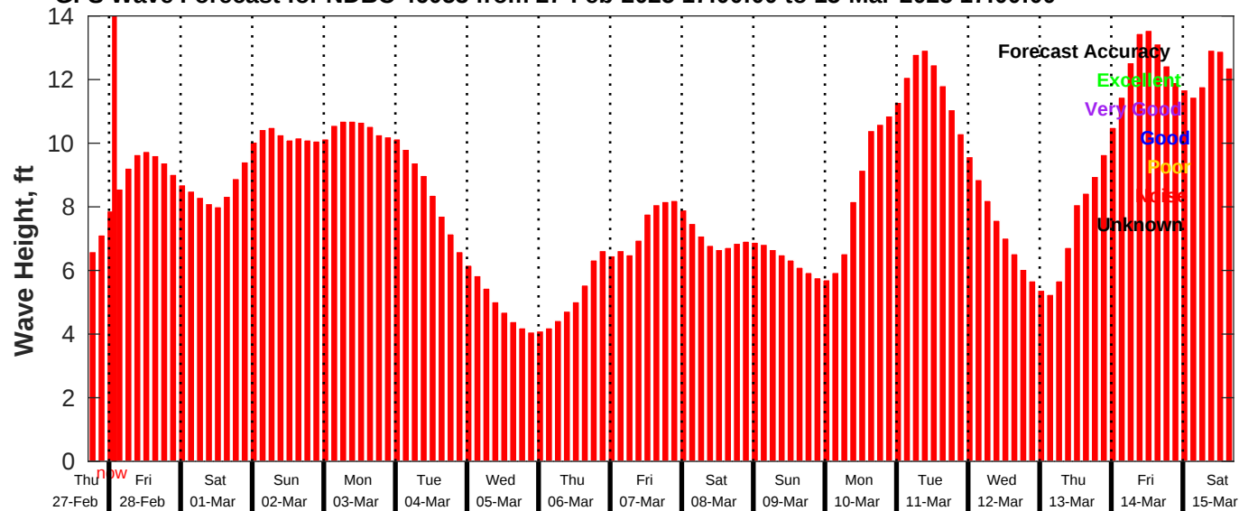
GFS Wave Forecast for NDBC 46053 from 27-Feb-2025 17:00:00 to 15-Mar-2025 17:00:00
