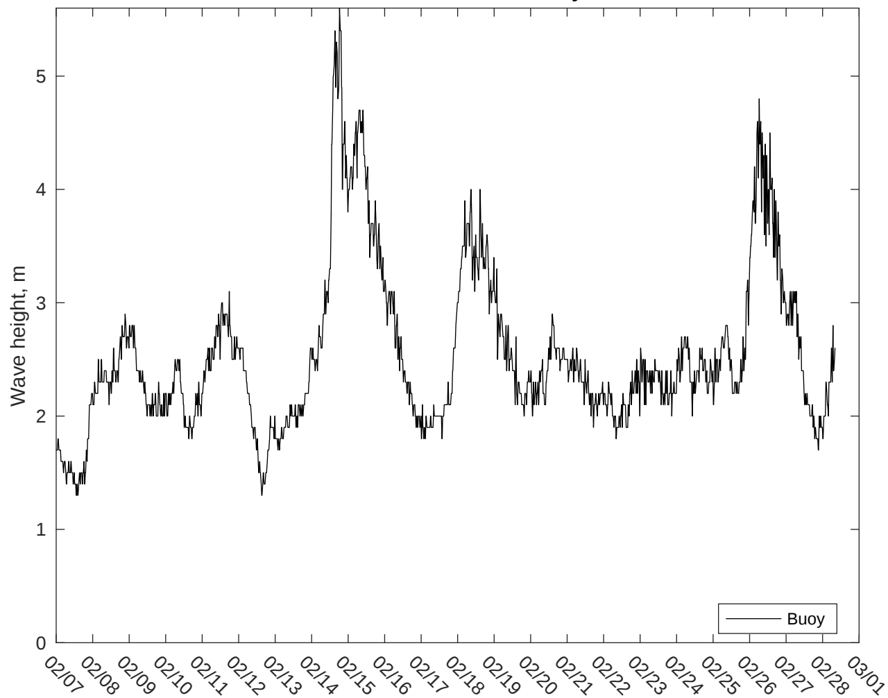
NDBC 46054 vs CMEMS Waves: 10 to 16 day forecast
