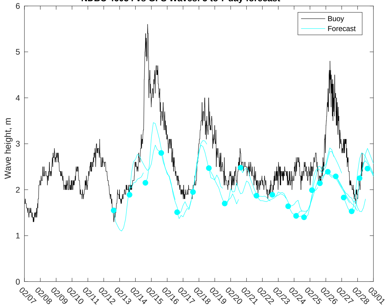
NDBC 46054 vs GFS Waves: 5 to 7 day forecast
