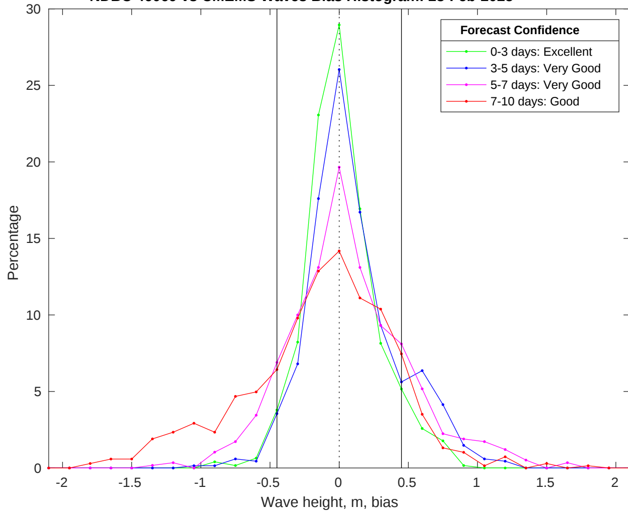
NDBC 46069 vs CMEMS Waves Bias Histogram: 28-Feb-2025
