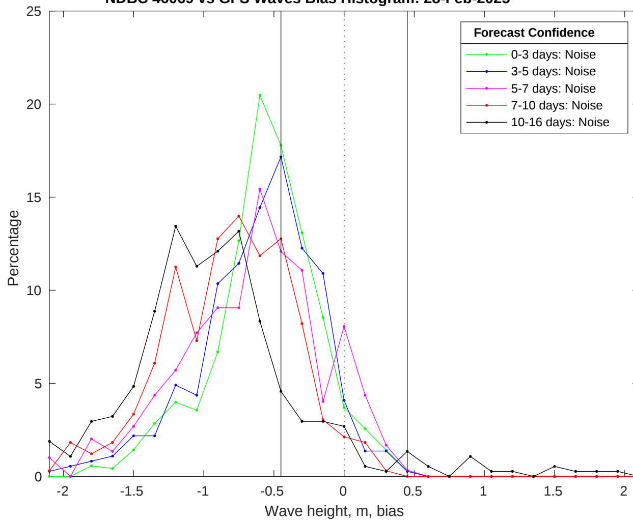
NDBC 46069 vs GFS Waves Bias Histogram: 28-Feb-2025
