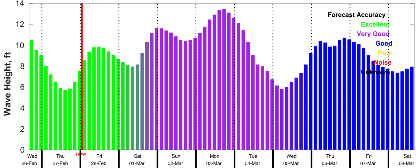
CMEMS Wave Forecast for NDBC 46069 from 26-Feb-2025 16:00:00 to 08-Mar-2025 16:00:00
