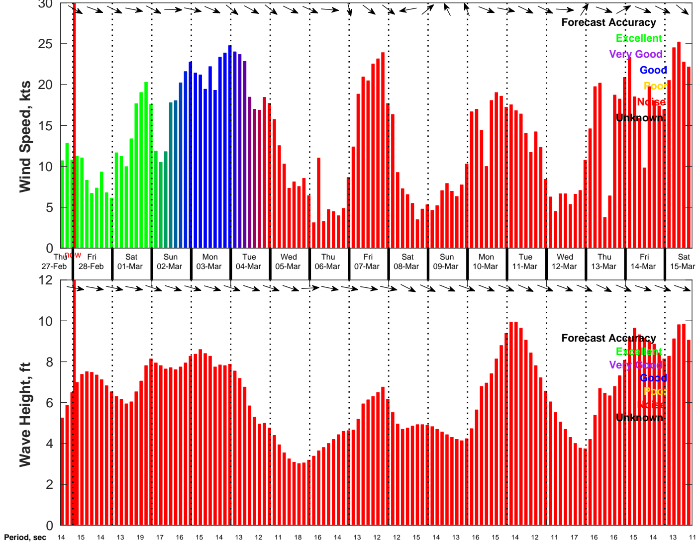
Wind & Wave Forecast for NDBC 46069 from 27-Feb-2025 16:00:00 to 15-Mar-2025 16:00:00
