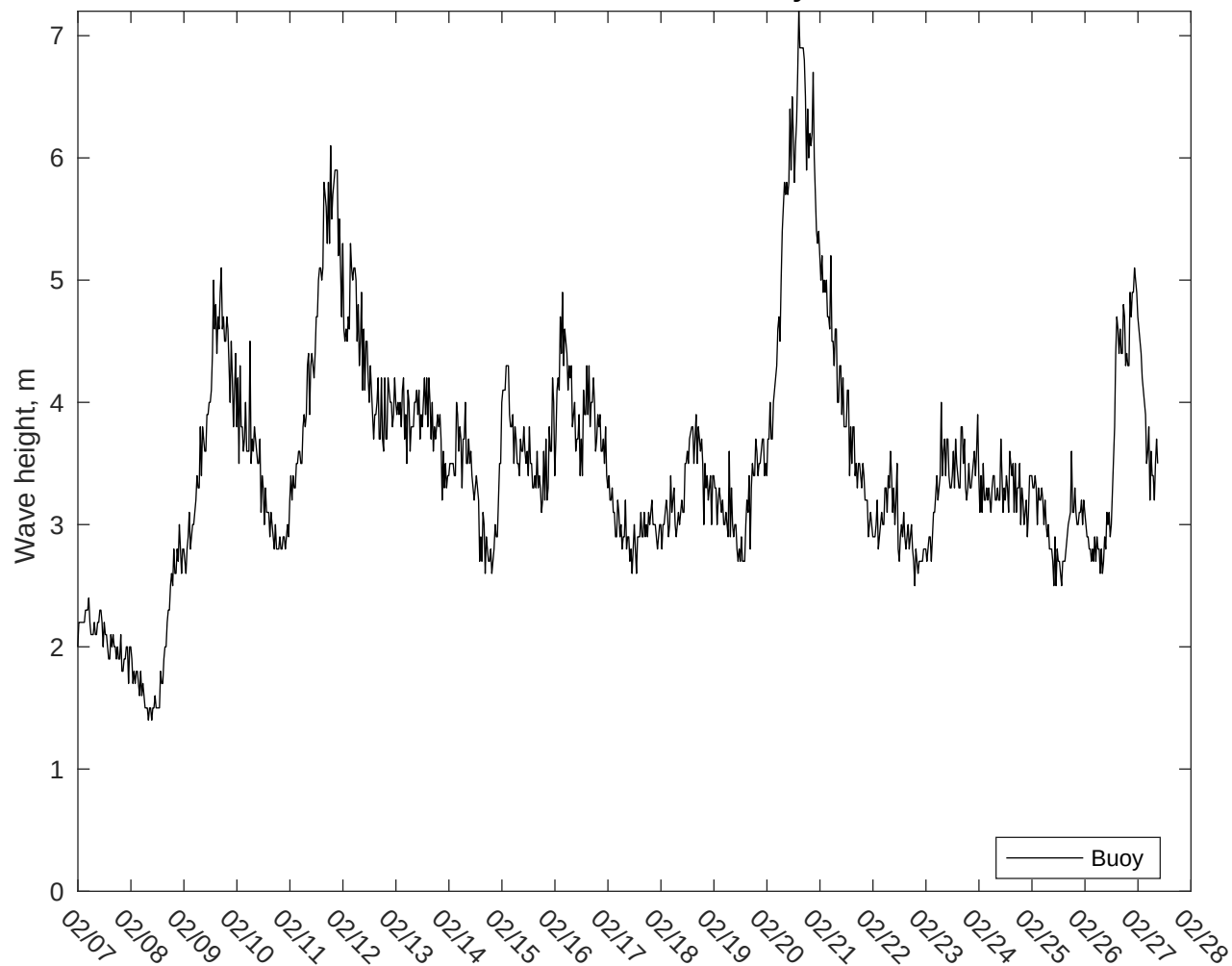
NDBC 46246 vs CMEMS Waves: 10 to 16 day forecast
