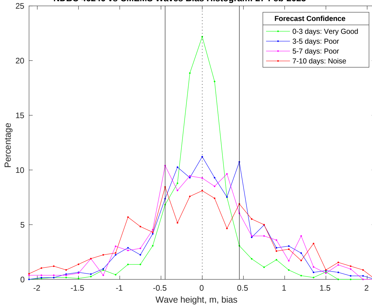
NDBC 46246 vs CMEMS Waves Bias Histogram: 27-Feb-2025
