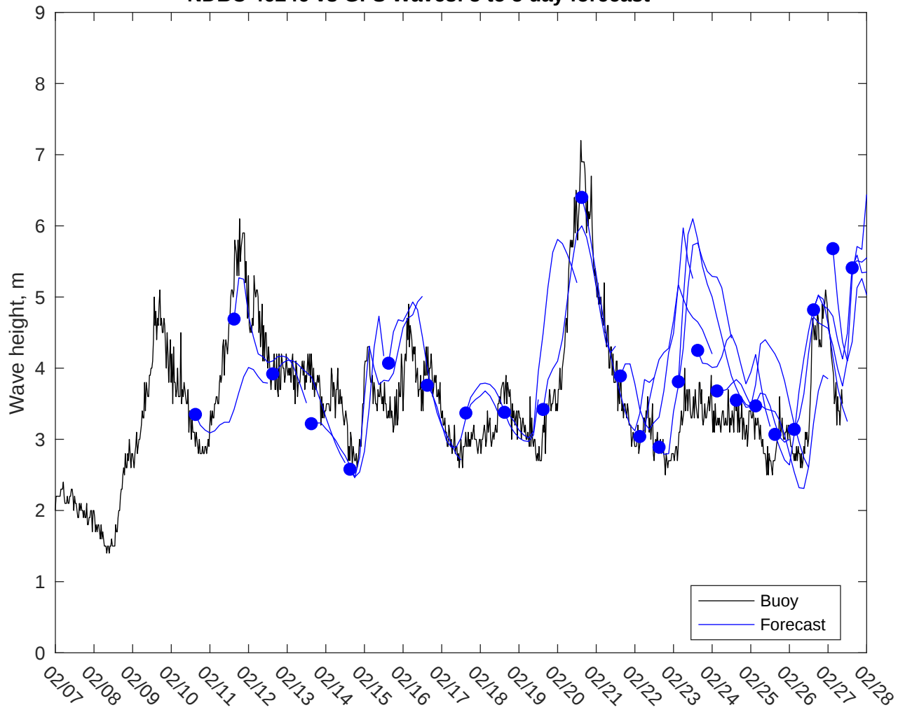
NDBC 46246 vs GFS Waves: 3 to 5 day forecast
