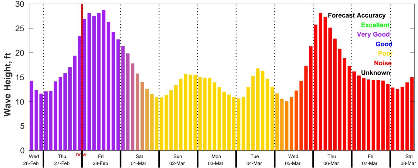
CMEMS Wave Forecast for NDBC 46246 from 26-Feb-2025 15:00:00 to 08-Mar-2025 15:00:00
