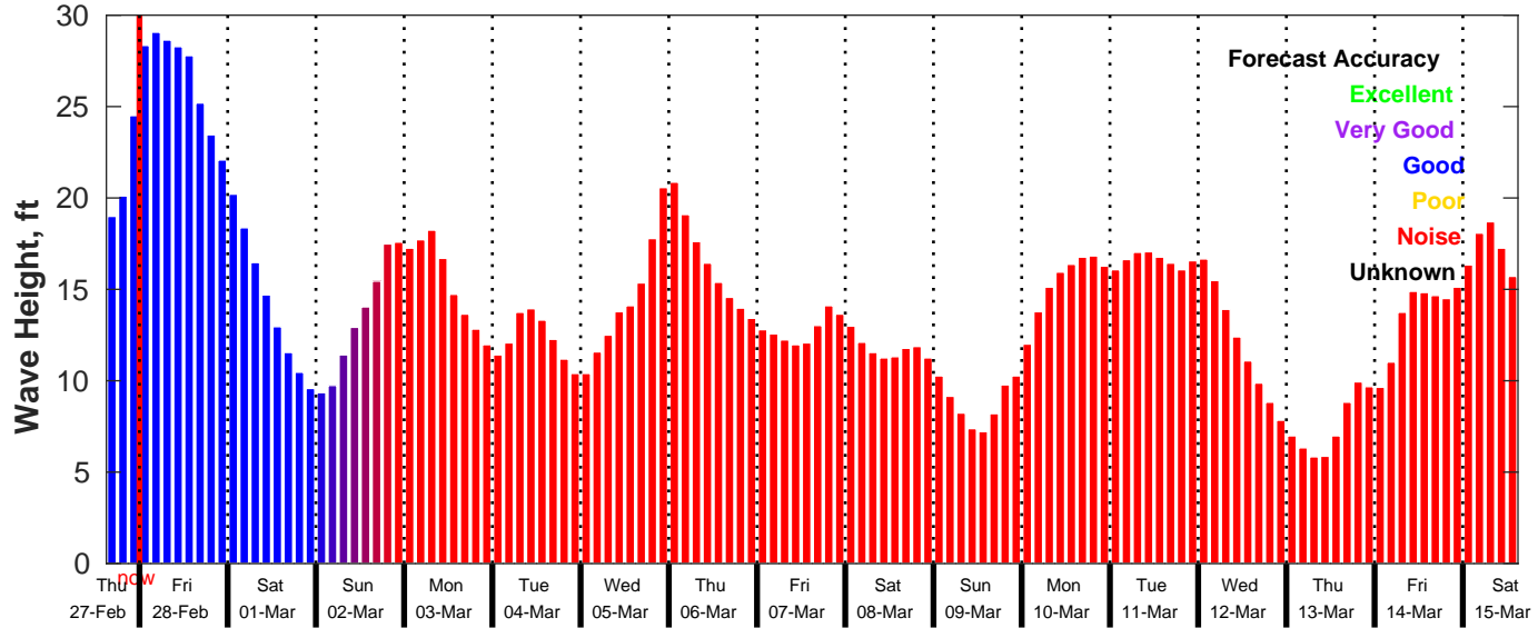
GFS Wave Forecast for NDBC 46246 from 27-Feb-2025 15:00:00 to 15-Mar-2025 15:00:00
