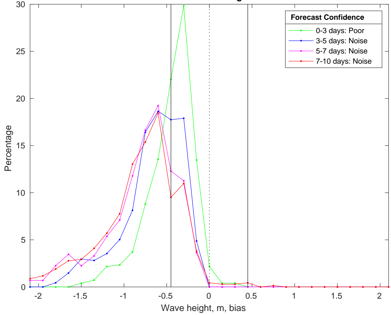
NDBC 51209 vs CMEMS Waves Bias Histogram: 28-Feb-2025
