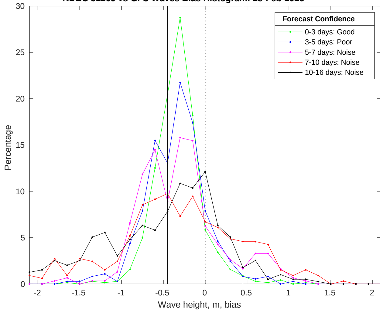
NDBC 51209 vs GFS Waves Bias Histogram: 28-Feb-2025
