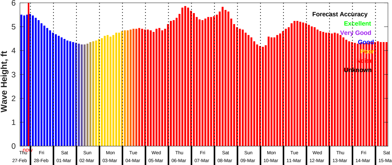
GFS Wave Forecast for NDBC 51209 from 27-Feb-2025 13:00:00 to 15-Mar-2025 13:00:00
