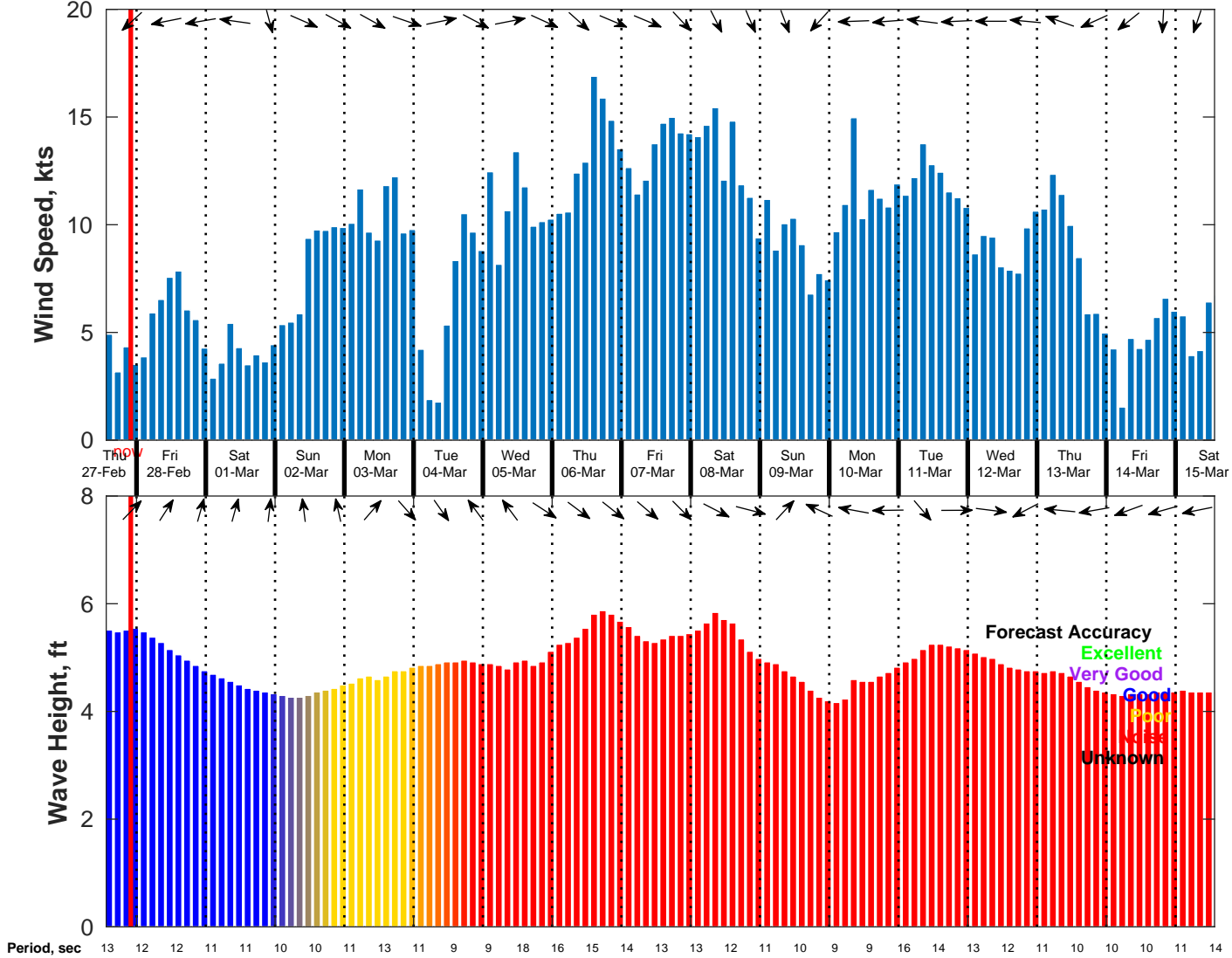
Wind & Wave Forecast for NDBC 51209 from 27-Feb-2025 13:00:00 to 15-Mar-2025 13:00:00
