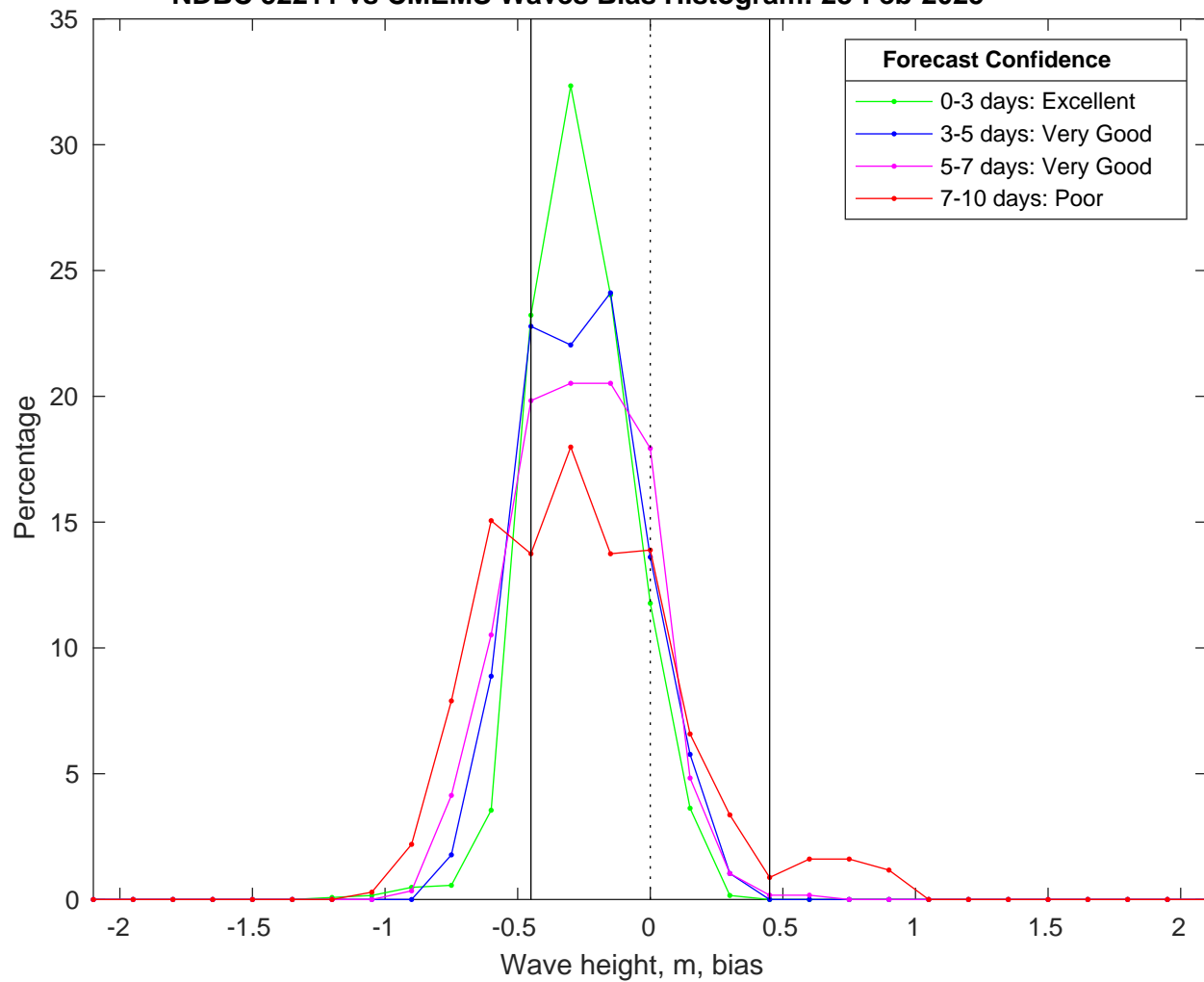
NDBC 52211 vs CMEMS Waves Bias Histogram: 28-Feb-2025
