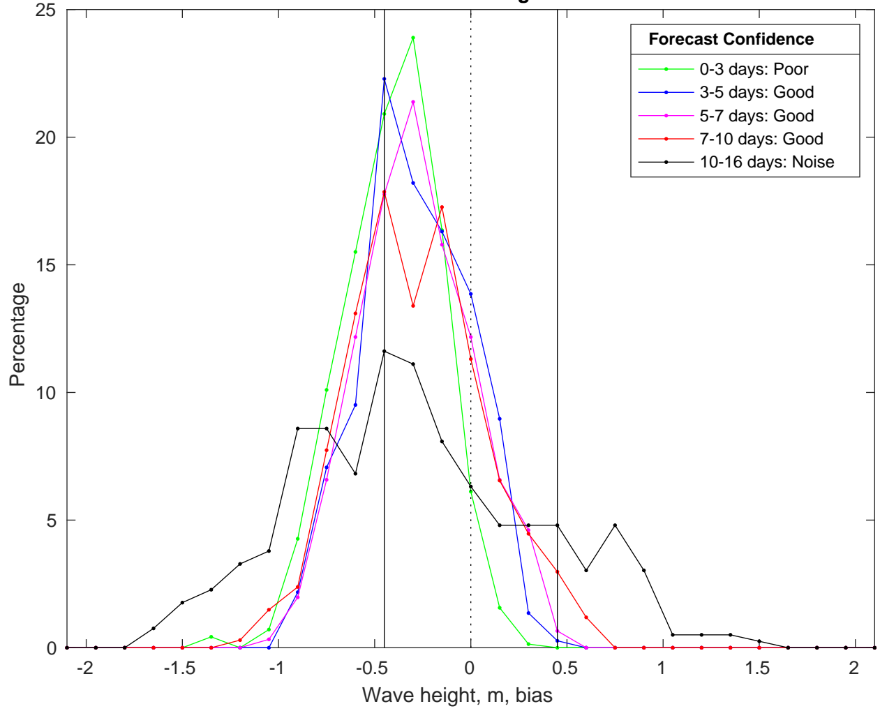
NDBC 52211 vs GFS Waves Bias Histogram: 28-Feb-2025
