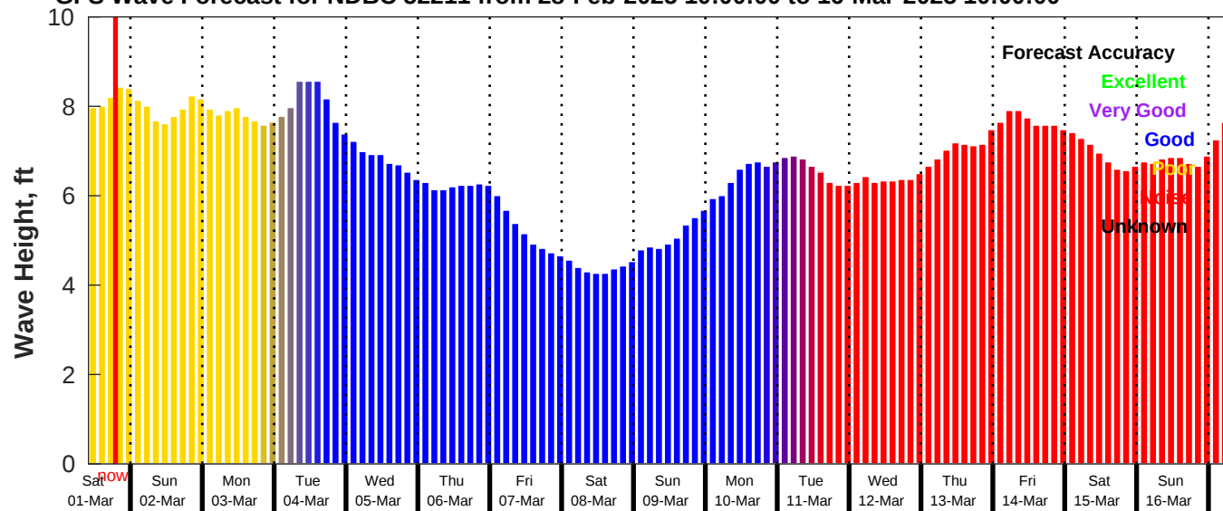
GFS Wave Forecast for NDBC 52211 from 28-Feb-2025 10:00:00 to 16-Mar-2025 10:00:00
