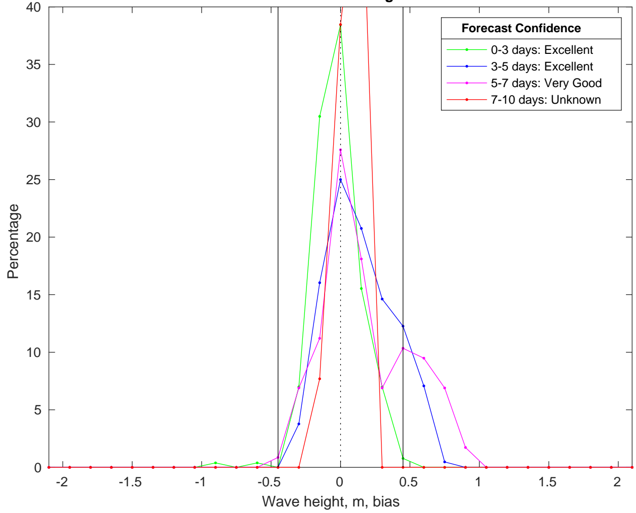
NDBC 52212 vs CMEMS Waves Bias Histogram: 28-Feb-2025
