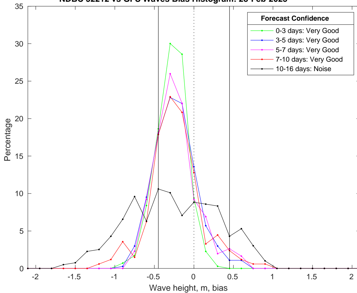
NDBC 52212 vs GFS Waves Bias Histogram: 28-Feb-2025
